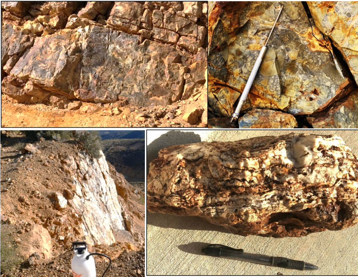
Upper left: pervasive silicification; upper right: hydrothermal breccia; lower left: epithermal vein viewed along strike; & lower right: crustiform banded vein.
